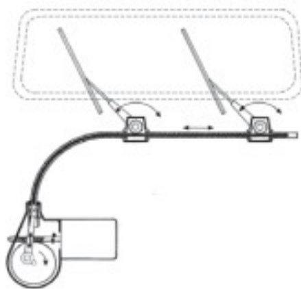
Schematic Windshield Wiper Motor
