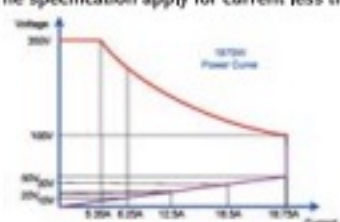
AEL-5002-350-18.75
