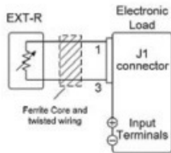
External Resistance Control
