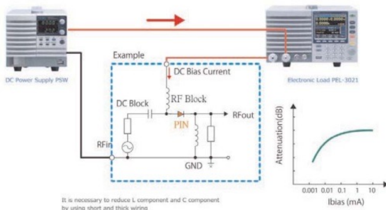
Bias Current vs. Attenuations
