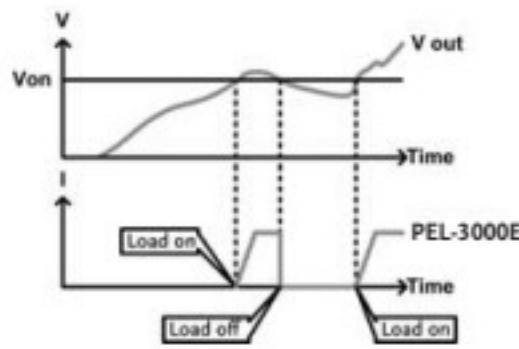
Von Latch = OFF
