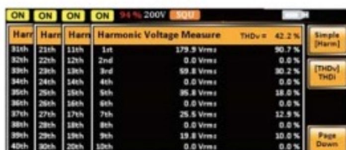
Voltage Harmonic
