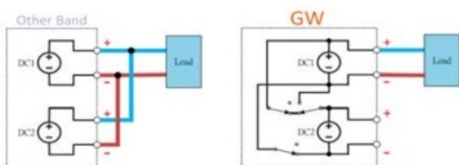
Output in Parallel Connections
