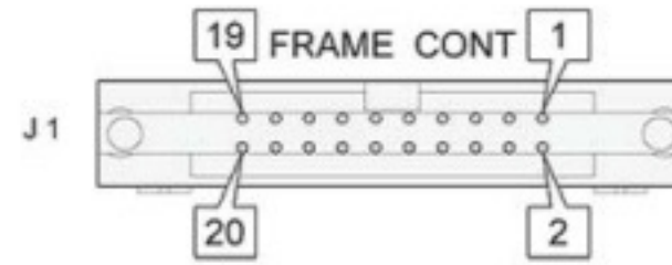
J1 Connector
