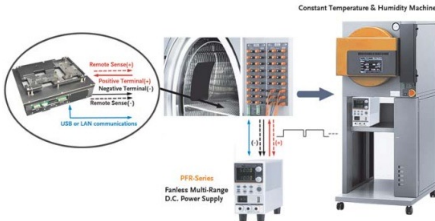
Schematic Diagram for Burn-in Test
