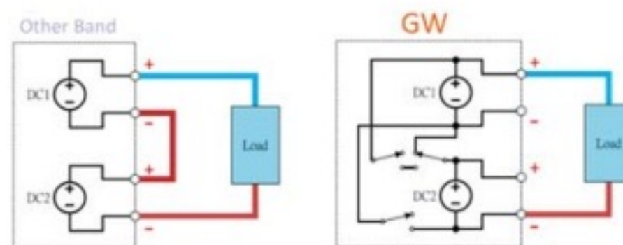
Output in Series Connections
