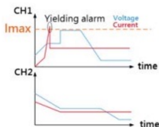
Output Monitoring
