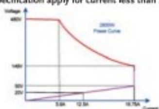
AEL-5003-480-18.75
