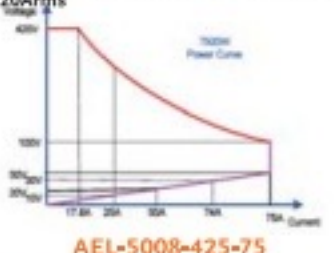
AEL-5008-425-75
