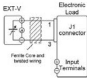
External Voltage Control
