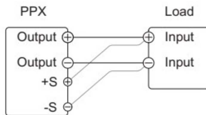
REMOTE SENSING CONNECTION DIAGRAM
