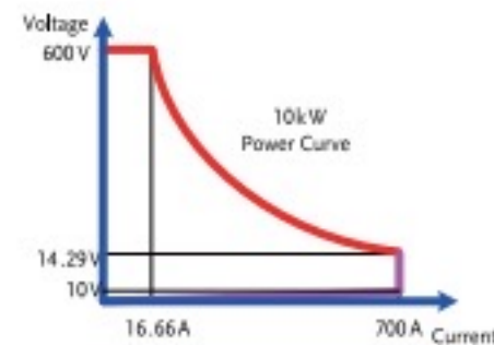
PEL-5010C-600-700
