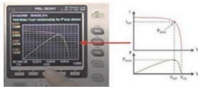
I-V Curve of The Solar Panel
