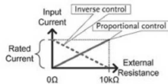
CC Mode
