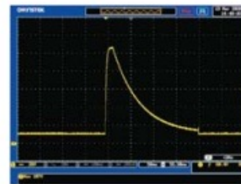
Load dump by ASR-2000 Series
