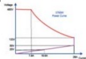
AEL-5004-480-28
