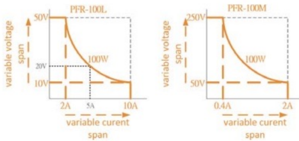
Voltage/Current Operating Area
