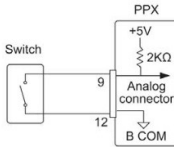
External Control of Output
