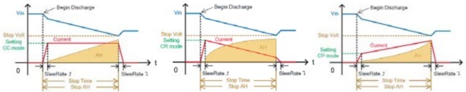
CC Mode
