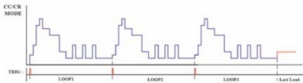
Fast Sequence Diagram
