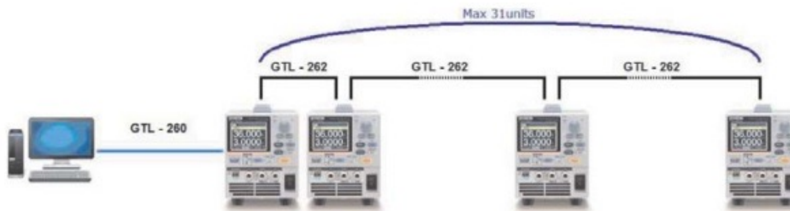
Multiple Unit Connection
