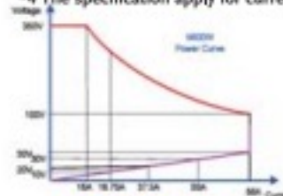
AEL-5006-350-56
