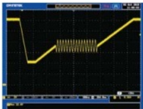
Starting profile by ASR-2000 Series
