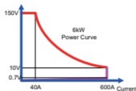
PEL-5006C-150-600
