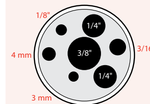
Multi-hole M06
