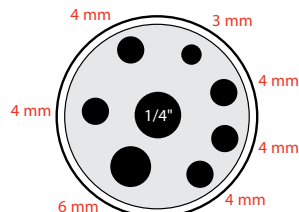
Multi-hole M01
