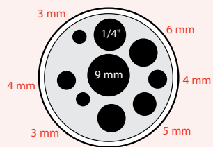
Multi-hole M04
