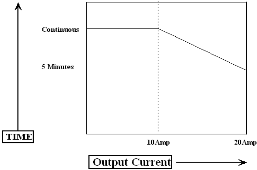
Graph 1* : Operating time on 22A range with current into a short circuit at 20°C Continuous current available up to 10A output.
