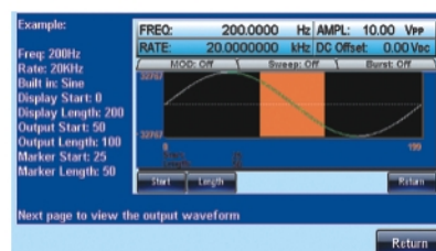
On-Screen Help
