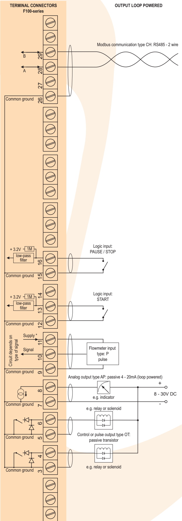
Typical wiring diagram F131-P-AP-CH-OT-PX
