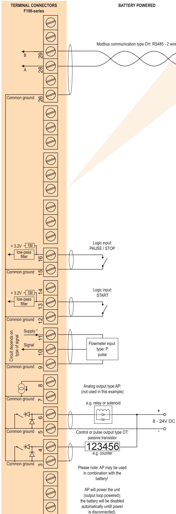
Typical wiring diagram F131-P-(AP)-CH-OT-PB
