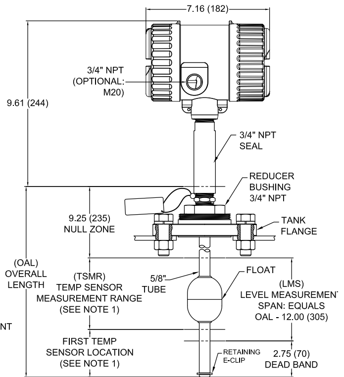
FIXED MOUNT (B2 STYLE)
