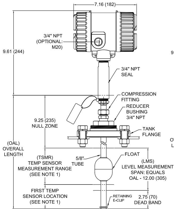
ADJUSTABLE MOUNT (B3 STYLE)
