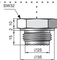
CM30×2 type M30×2 with flush Diaphragm
